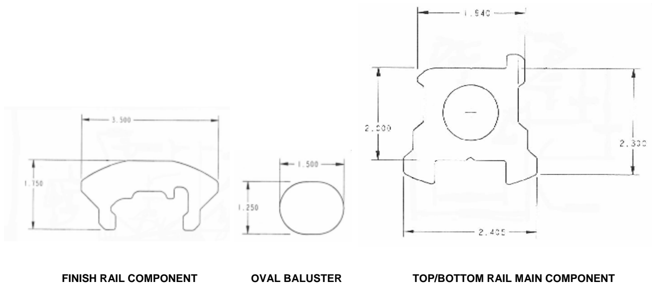
FIGURE 2—EPOCH EVERGRAIN TRADITIONAL RAILING AND 2x4 TRADITIONAL RAILING COMPONENT CROSS SECTIONS
